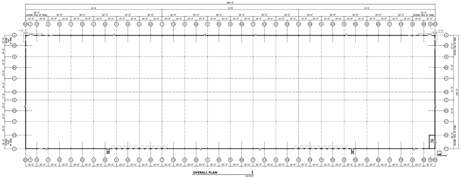
OVERALL PLAN 1 1/8"=1'-0"
